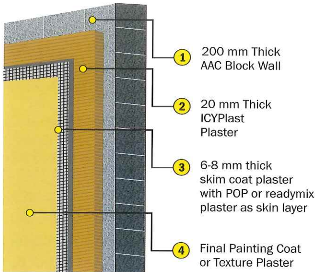
IcyPlast Wall Treatment (Typical Cross-Section)
